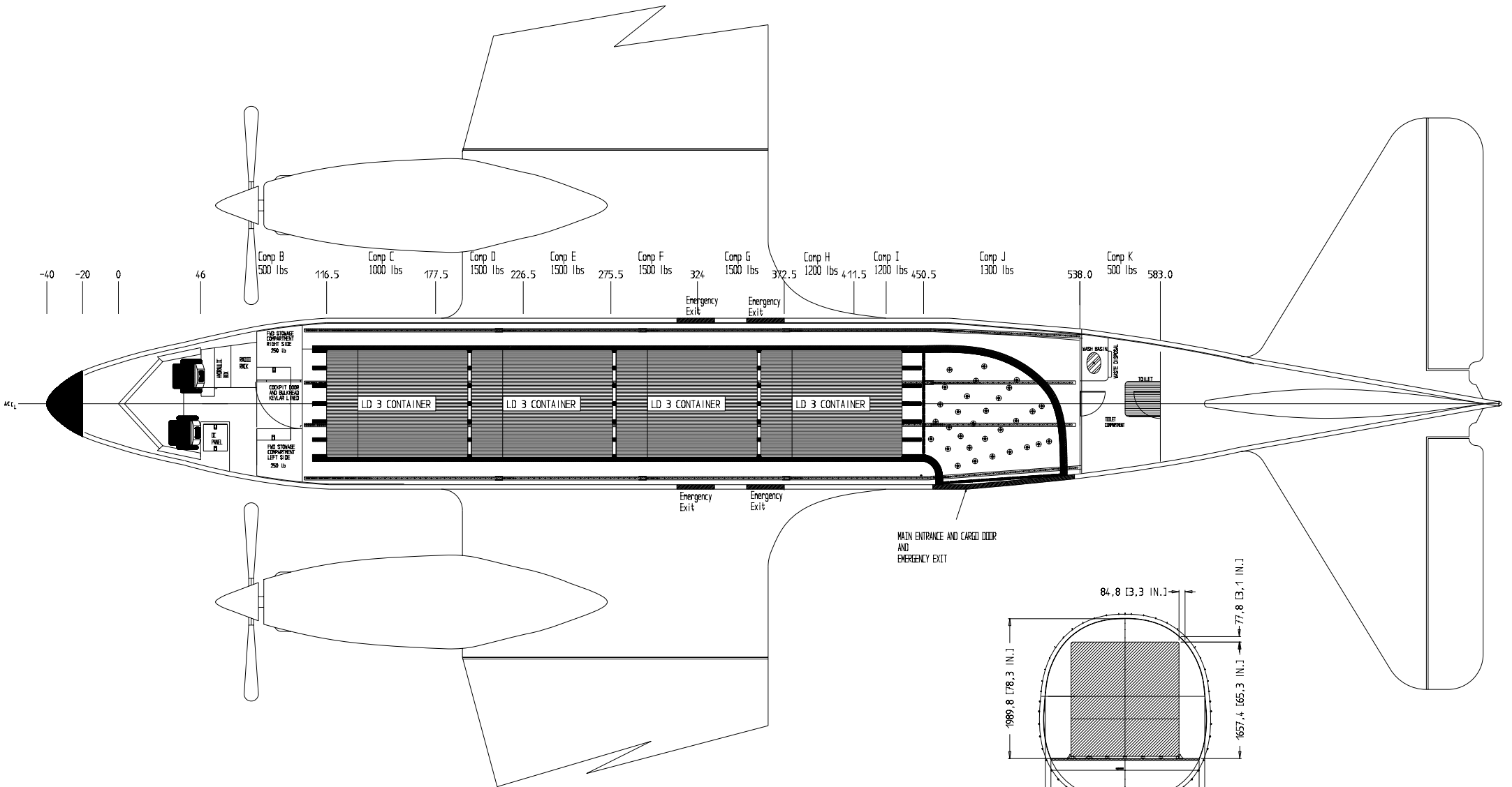
DC3/C47-65ARTP AIRCRAFT: LD3 CARGO CONTAINER CONFIGURATION
